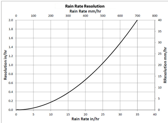
Figure 1. Rain Rate Resolution
