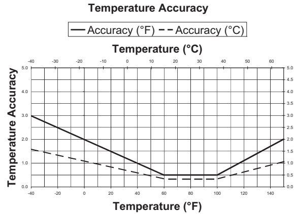
Figure 2: External Temperature Probe Accuracy
